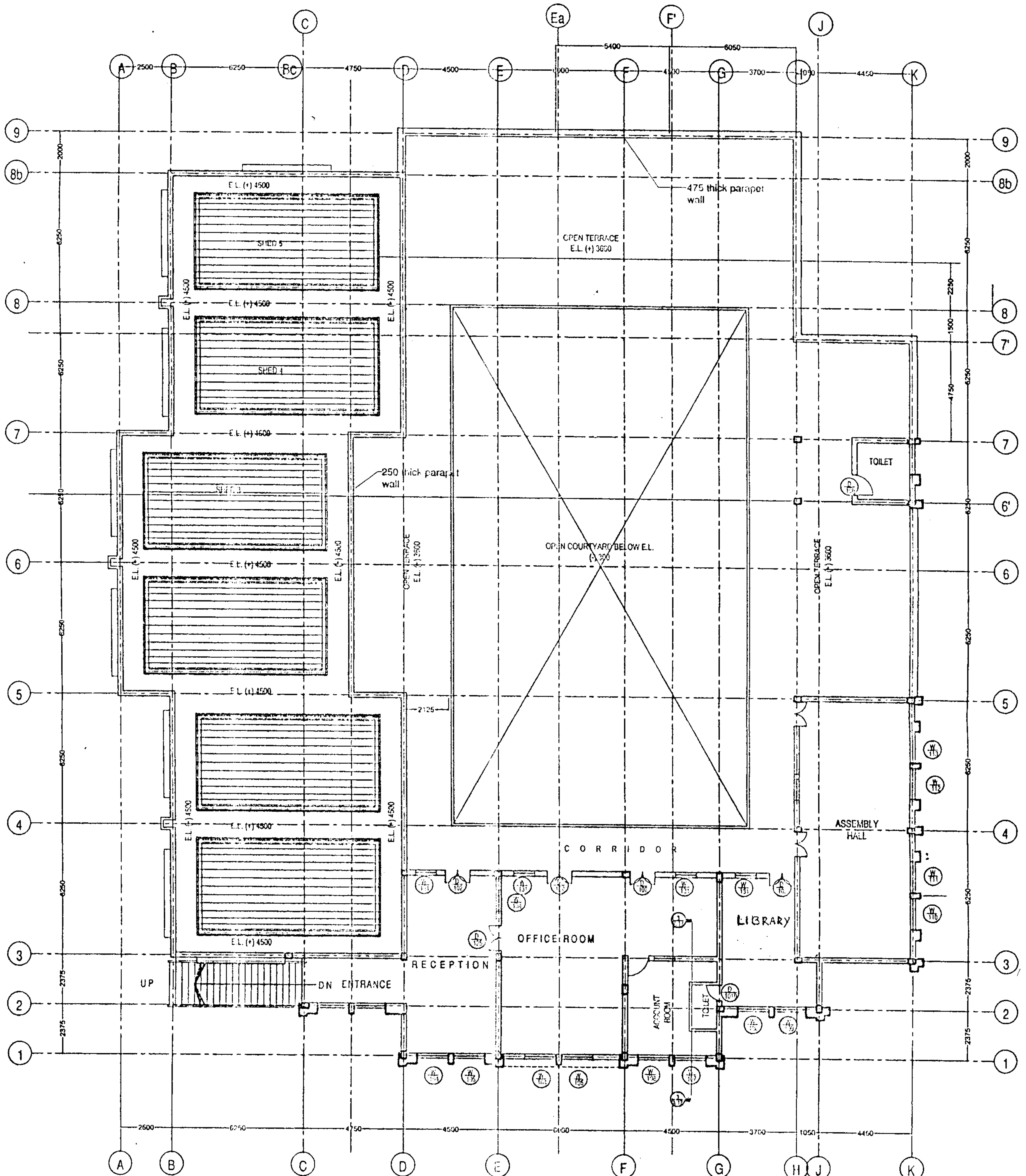
ROOF PLAN/ FIRST FLOOR PLAN
